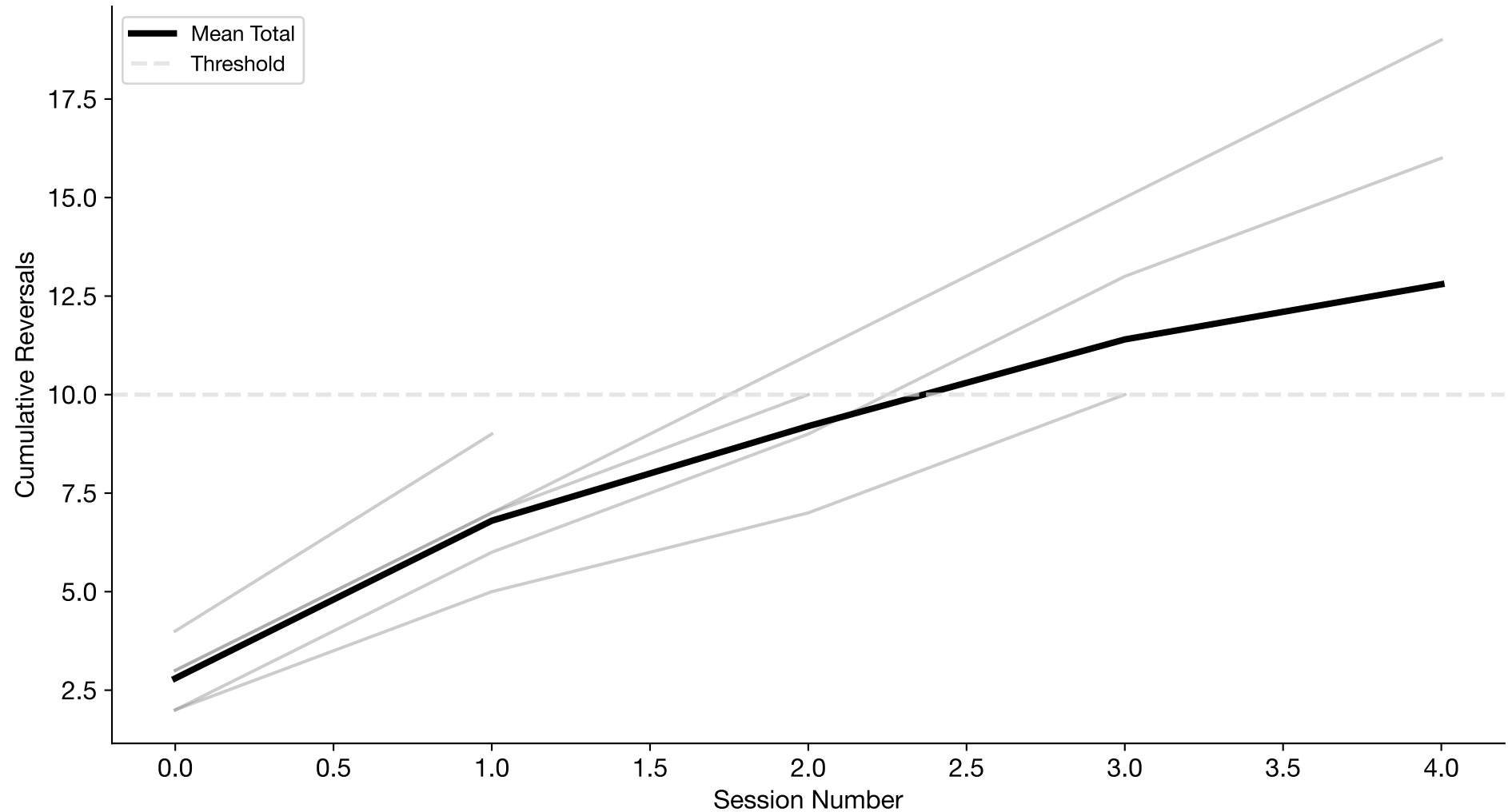
Cumulative Total Reversals Over Time (n=5 subjects; sessions per subject=2–5)
